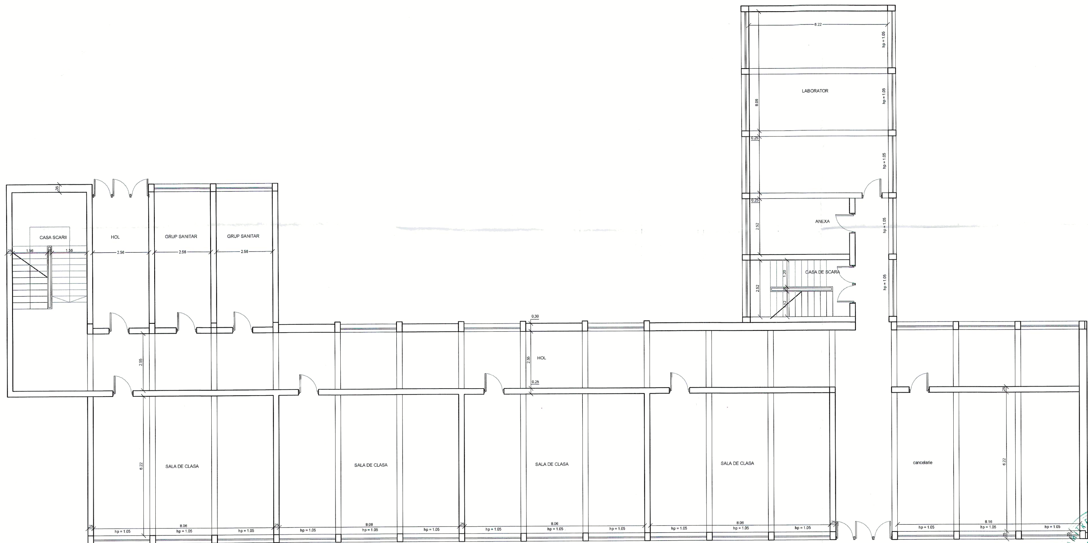
PLAN PARTER
